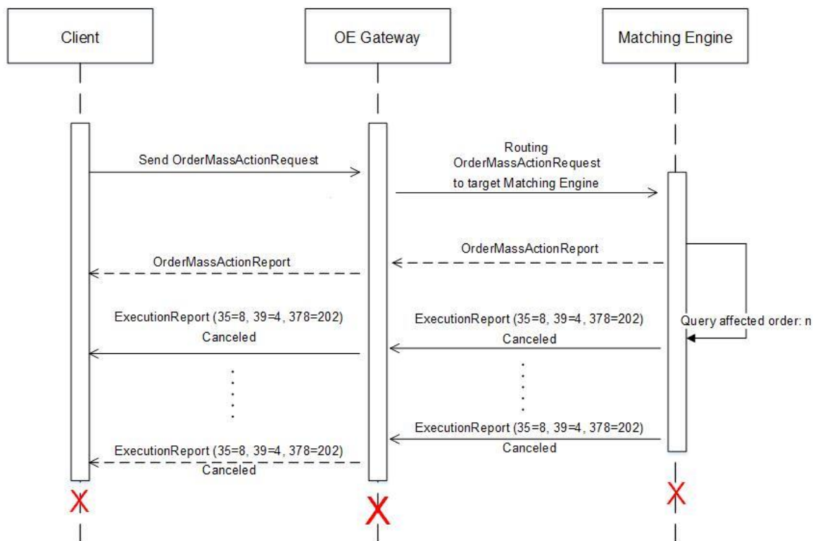
Figure 12 – Session Level Cancel
