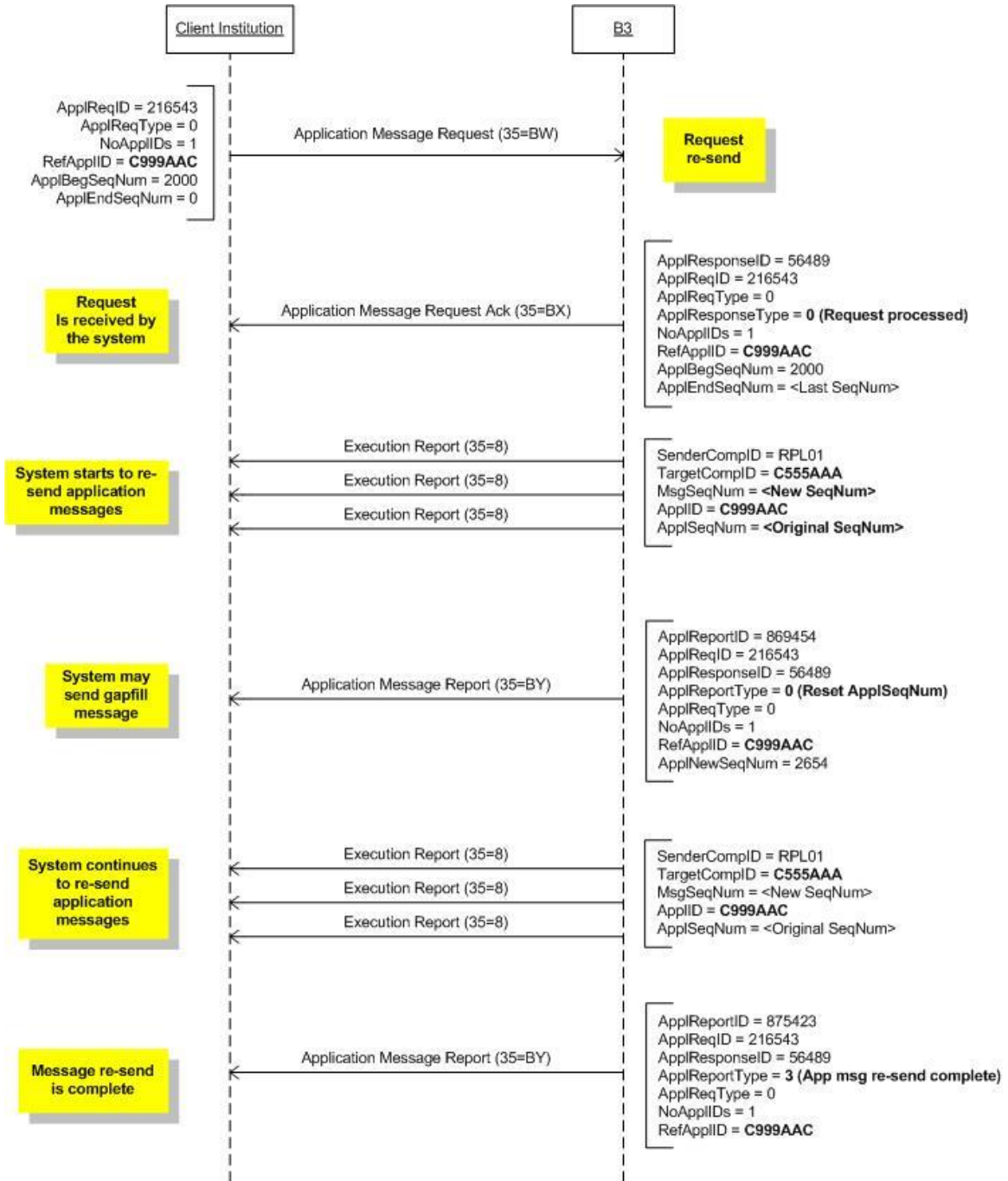
Figure 53 - Message Re-send
