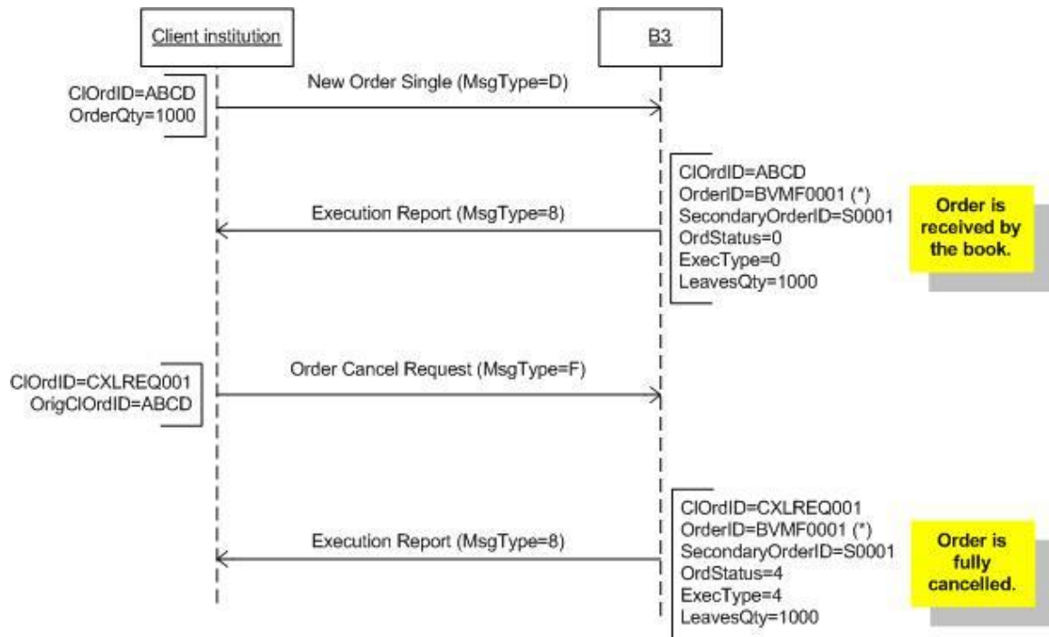
Figure 8 - Order cancellation using CIOrdID
