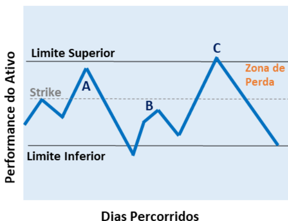
Double No Touch+ Call Digital
