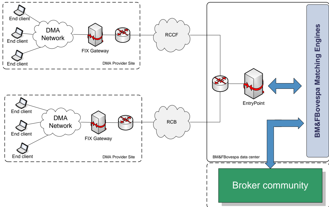
Figure 1 - B3 DMA providers' network setup
